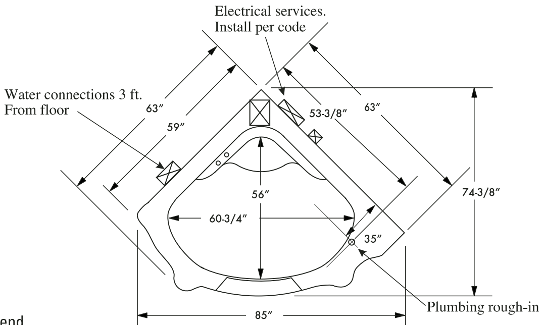
PLAN VIEW
