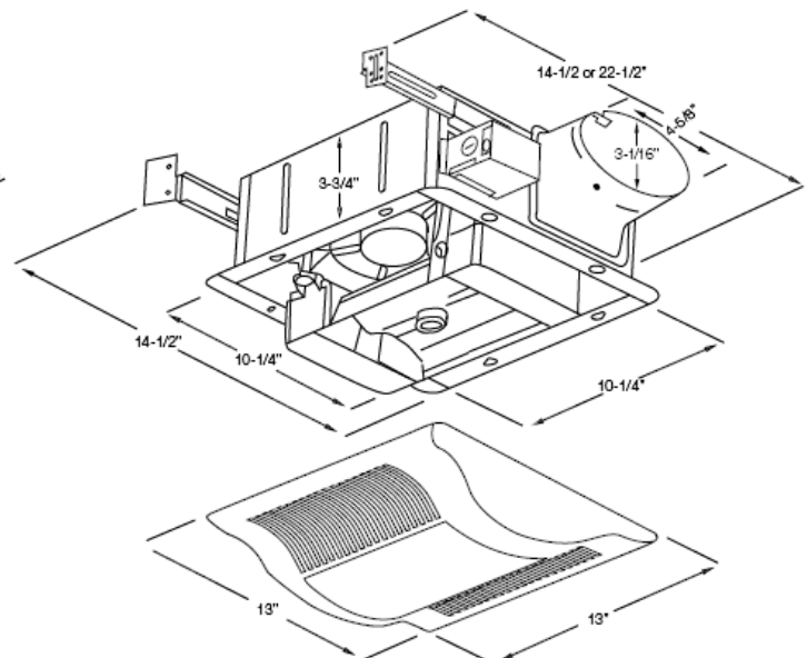
FV-10VSL1 4" oval duct
