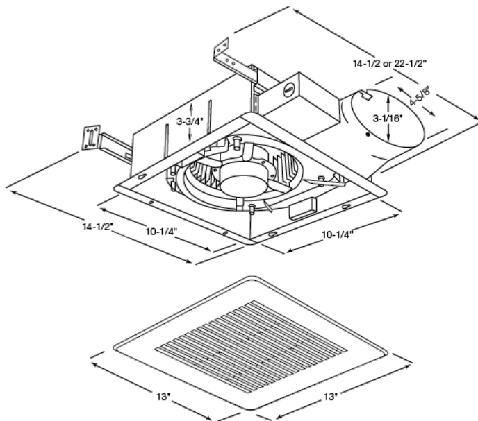
FV-10VS1 4" oval duct
